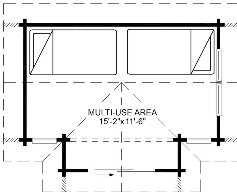
MAIN FLOOR 160 square feet (14.90 m 2 )
