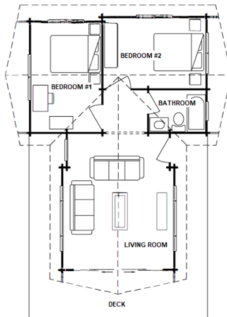
MAIN FLOOR 650 square feet (60.37 m²)
