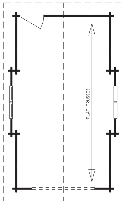
MAIN FLOOR 285 square feet (26.44 m 2 )
