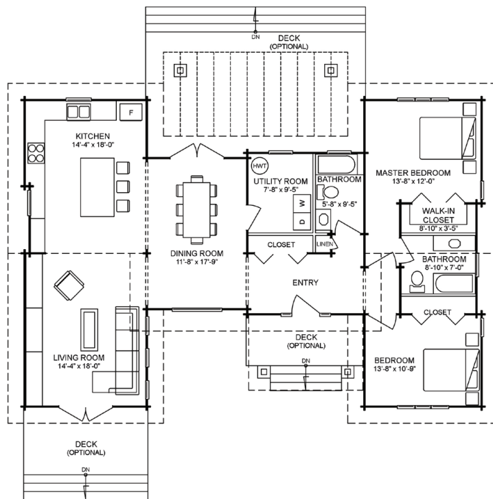
MAIN FLOOR
