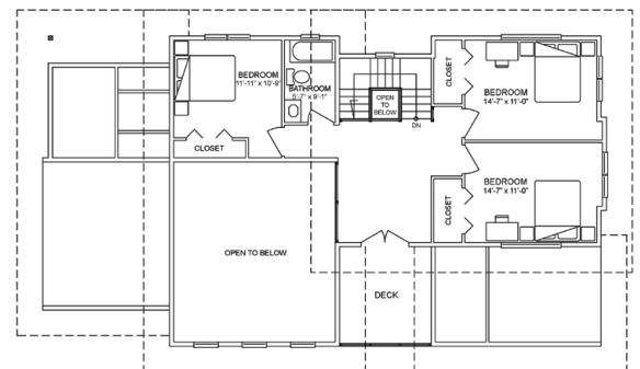
UPPER FLOOR 858 square feet (79.71 m 2 )
