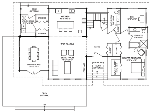
MAIN FLOOR 1,888 square feet (175.40 m 2 )
