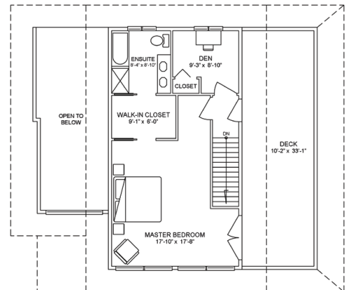
UPPER FLOOR 600 square feet (55.74 m 2 )
