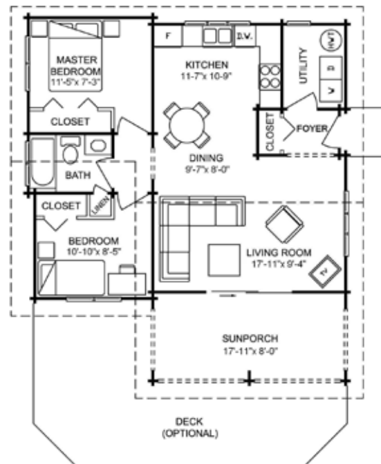
MAIN FLOOR 777 square feet (72.18 m²)
