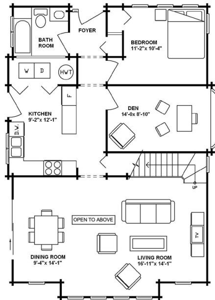
MAIN FLOOR
