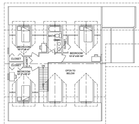
UPPER FLOOR 714 square feet (66.31 m 2 )
