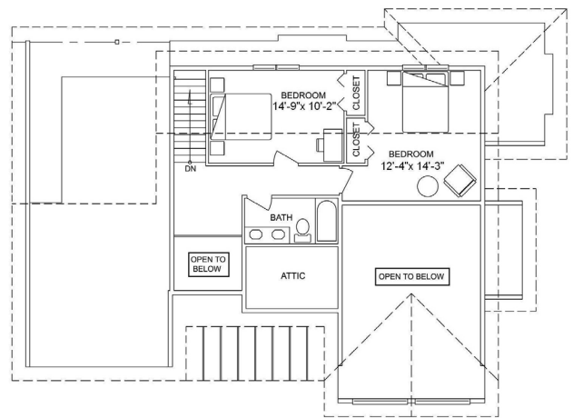
UPPER FLOOR 558 square feet (51.82 m 2 )
