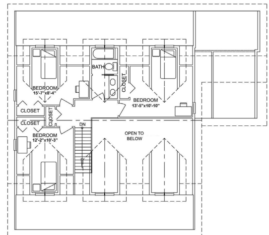
UPPER FLOOR 714 square feet (66.31 m 2 )
